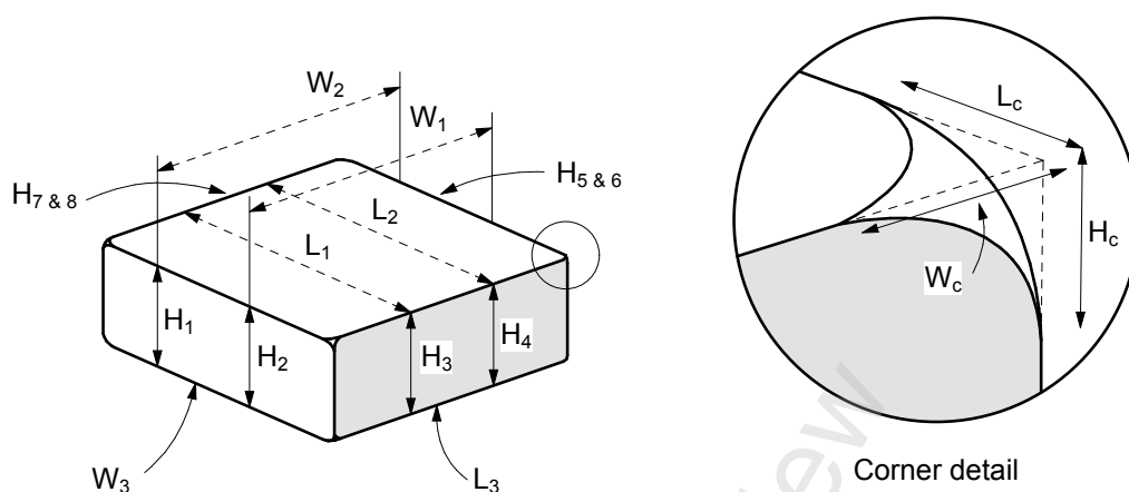
Figure M1 – Measurement of block for density measurement
