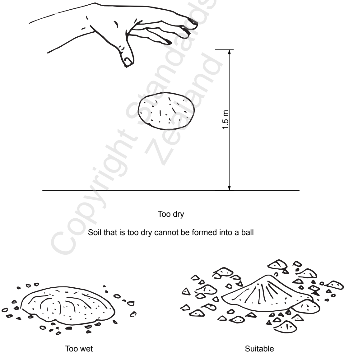
Figure I1 – Moisture content for rammed earth
