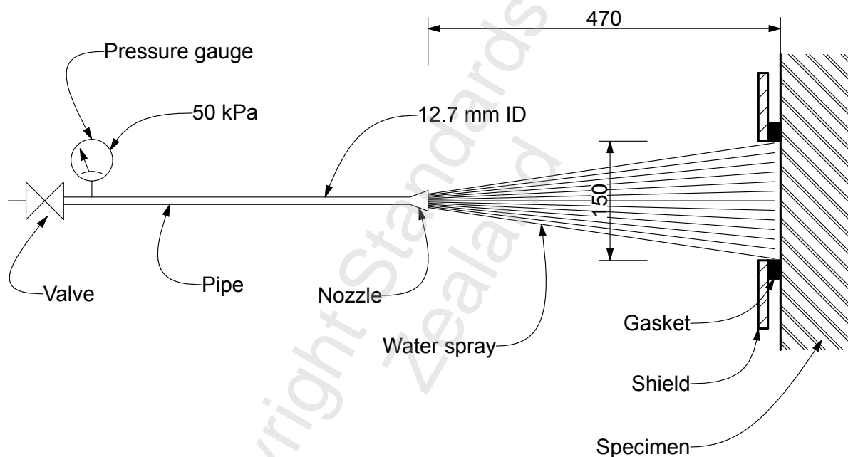
Figure K1 – Pressure spray test general arrangement
