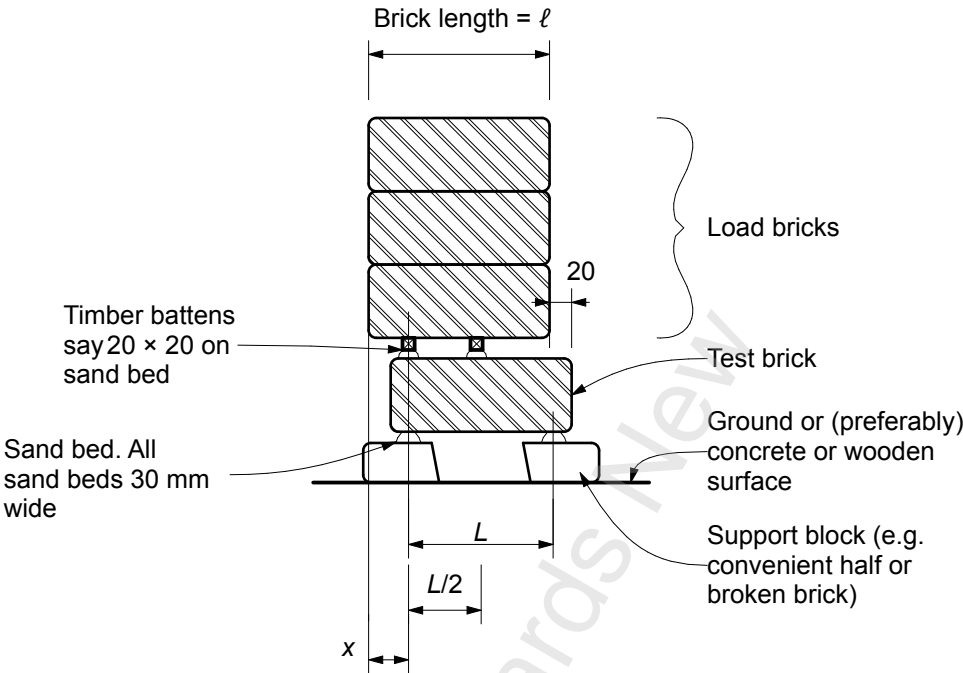
Figure G1 – Stacked bricks rupture test
