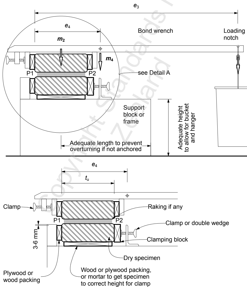
DETAIL A
