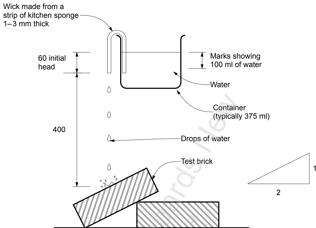
Figure L1 – Drip erosion test method erosion test configuration
