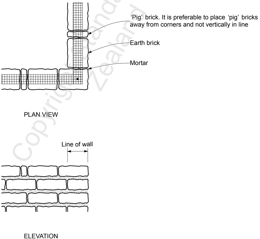
Figure 5.1 – Brick bond
