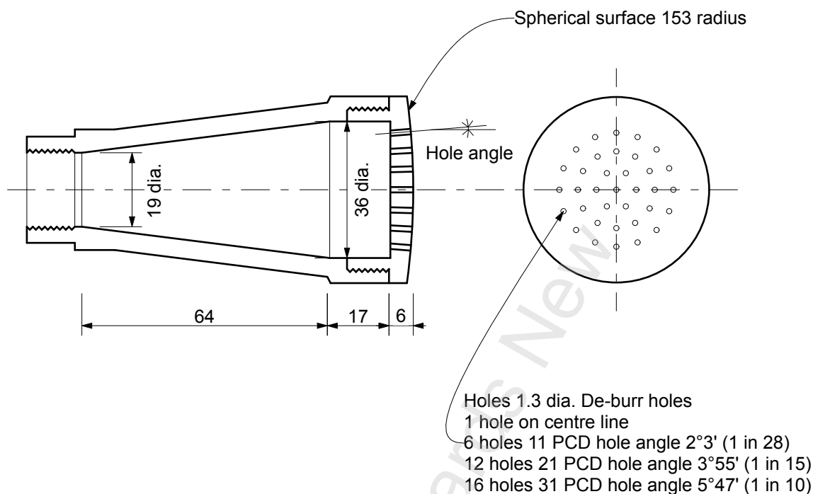
Figure K2 – Pressure spray test nozzle
