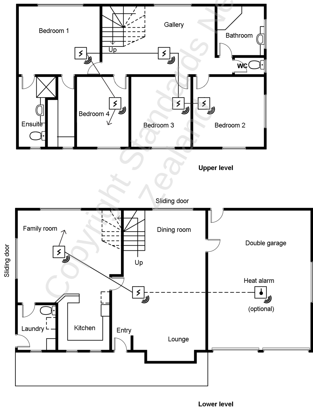
Figure B4 – Multi-level house floor plans
