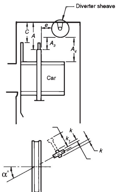
Figure 9.3.3 – Clearances above the car where overload diverter sheave protrudes below liftwell ceiling
