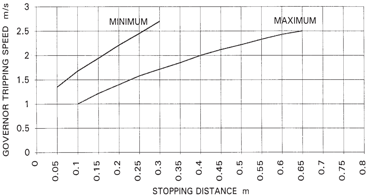
(b) Governor tripping speeds < 2.5 m/s
