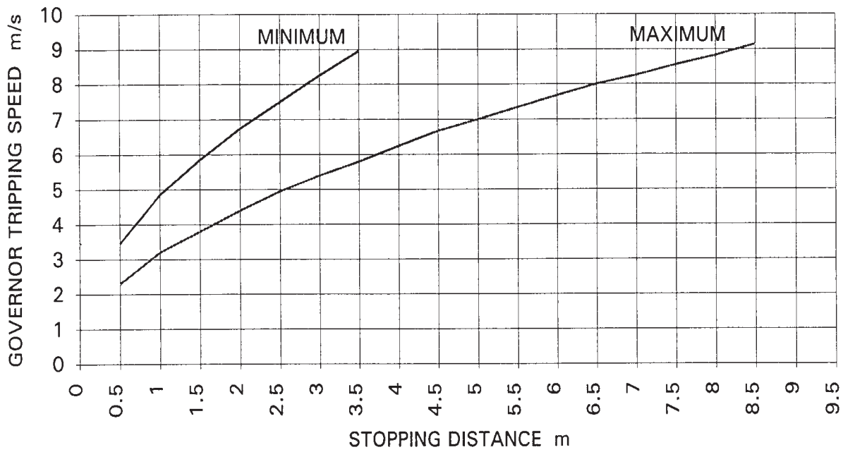
(a) Governor tripping speeds > 2.5 m/s
