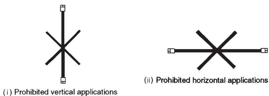
Figure 35.3.5 (b) – Prohibited practices for positioning hydraulic hoses
