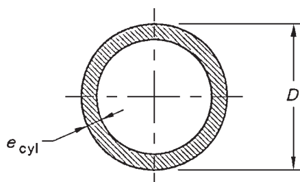
DIMENSIONS IN MILLIMETRES
