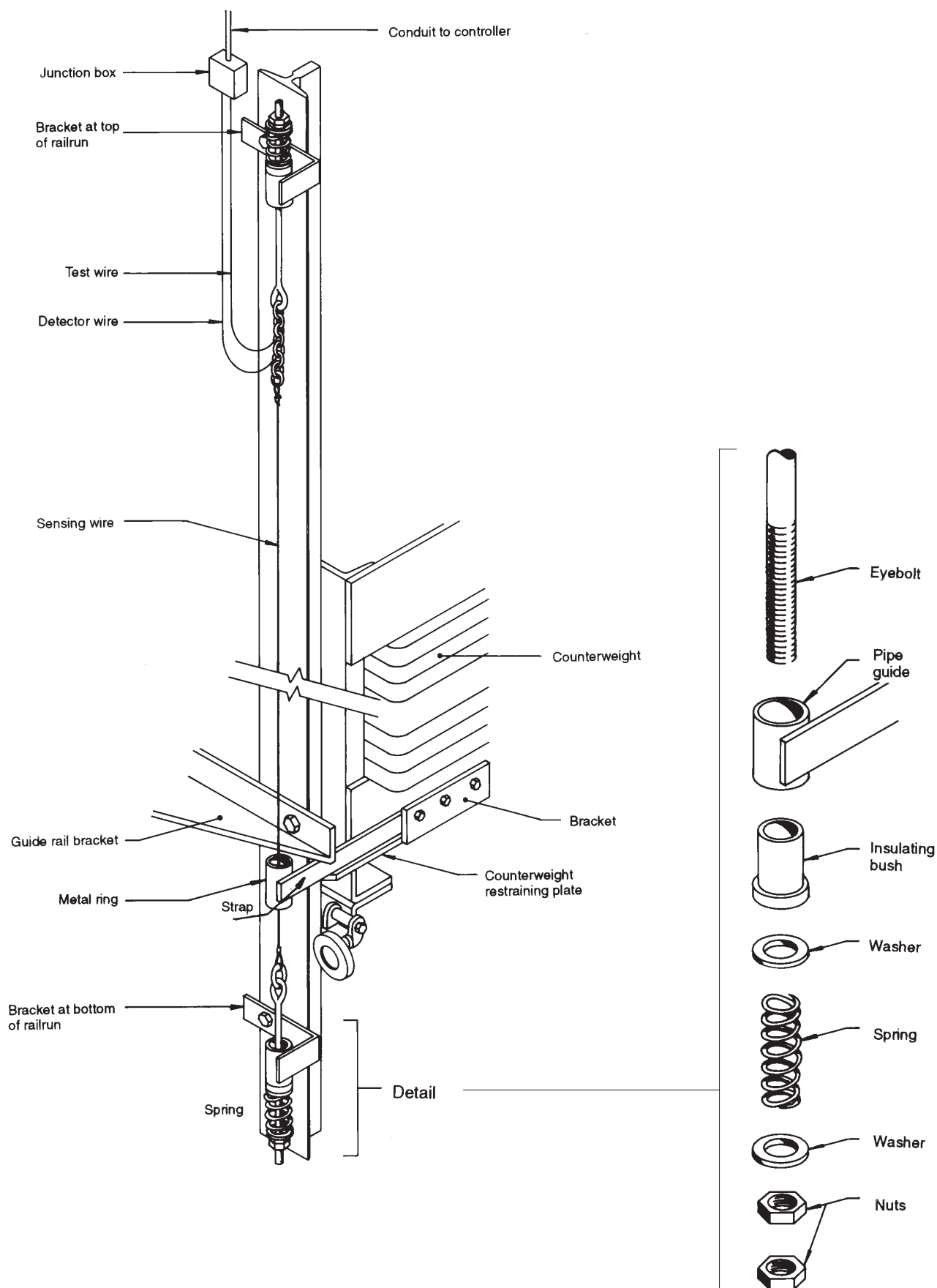
Figure 25.1 – Major component displacement detector
