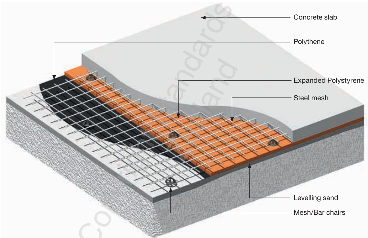
Figure 36 – Under-slab insulation
