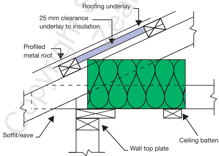
Figure 25 – Profiled metal roof
