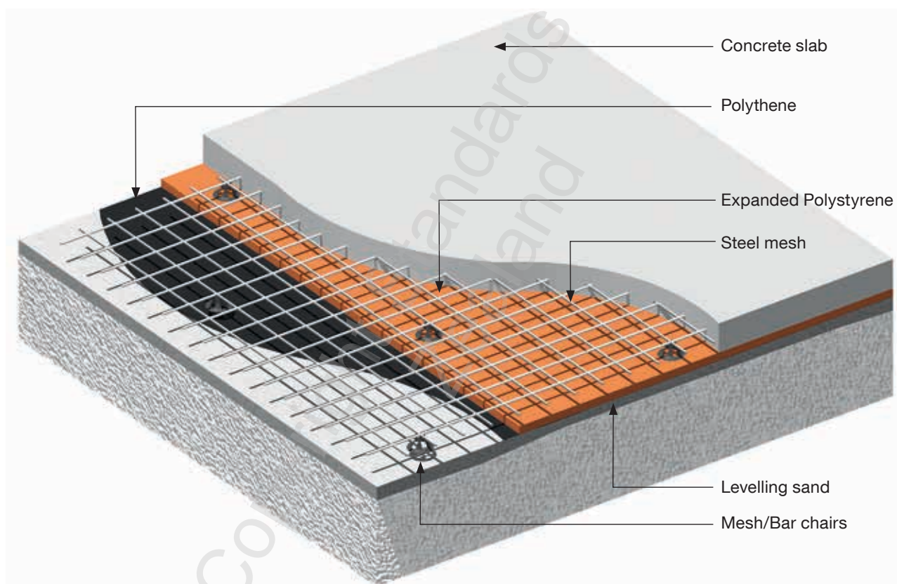
Figure 36 – Under-slab insulation
