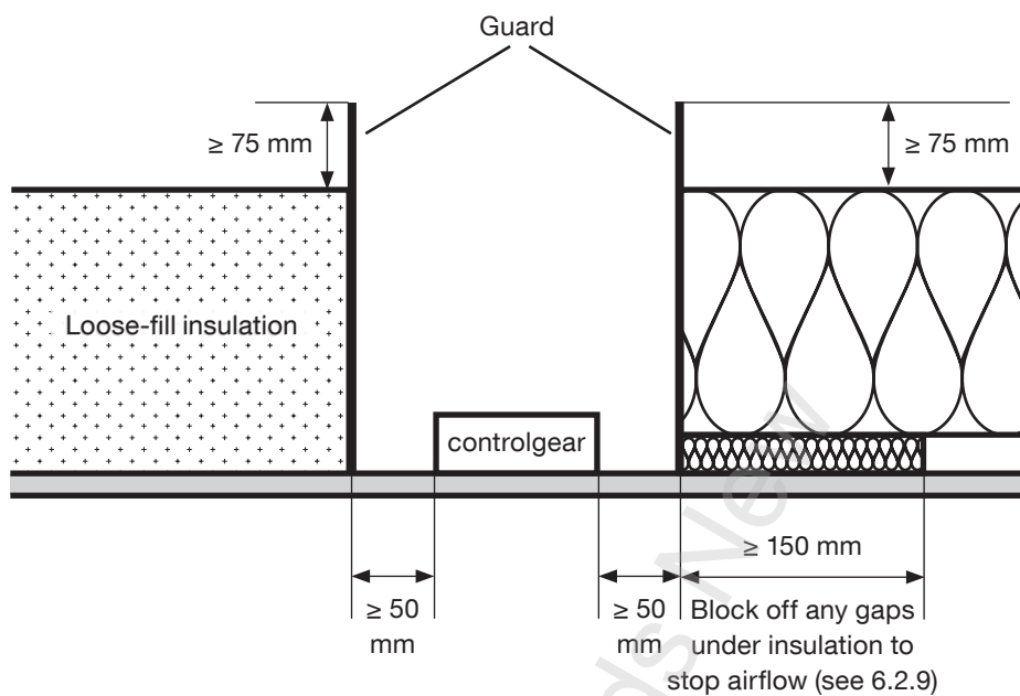
Figure 15 – Example of ceiling insulation clearance around independent controlgear not placed on top of insulation, where the manufacturer’s instructions are not known
