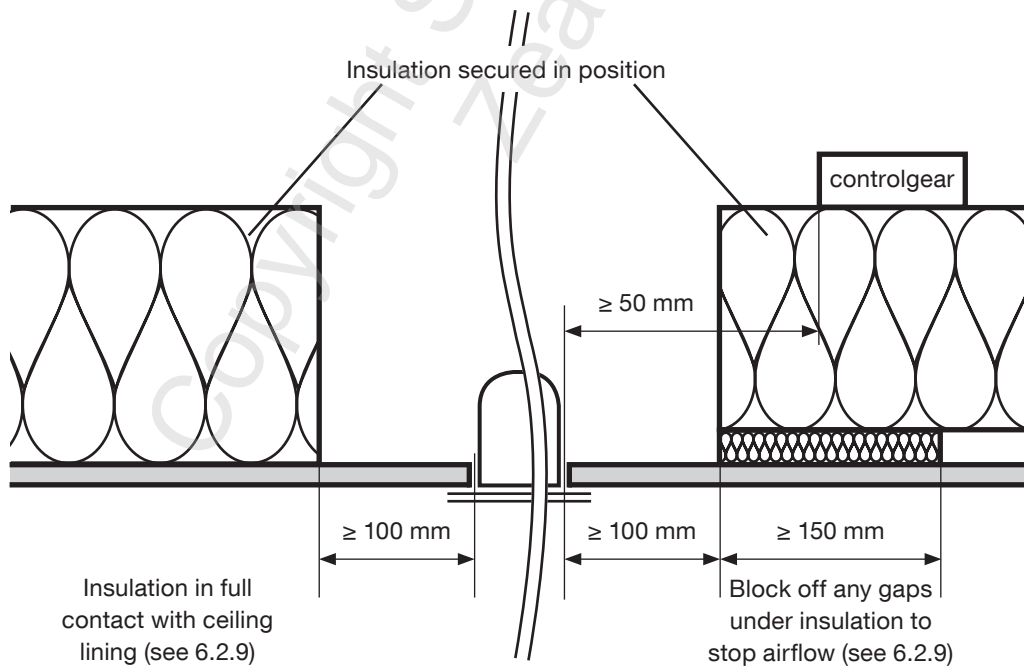
Figure 9 – Installing ceiling insulation around recessed luminaires that are NOT of the type CA 80, CA 90, CA 135, IC, IC-F, or IC-4 where insulation is secured in position and where the luminaire manufacturer’s instructions are not known
