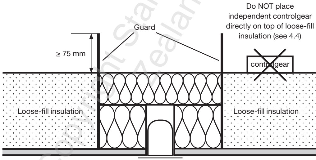
Figure 7 – Installing new loose-fill ceiling insulation around recessed luminaires of the type IC, IC-F, and IC-4 where the luminaire manufacturer’s instructions are not known
