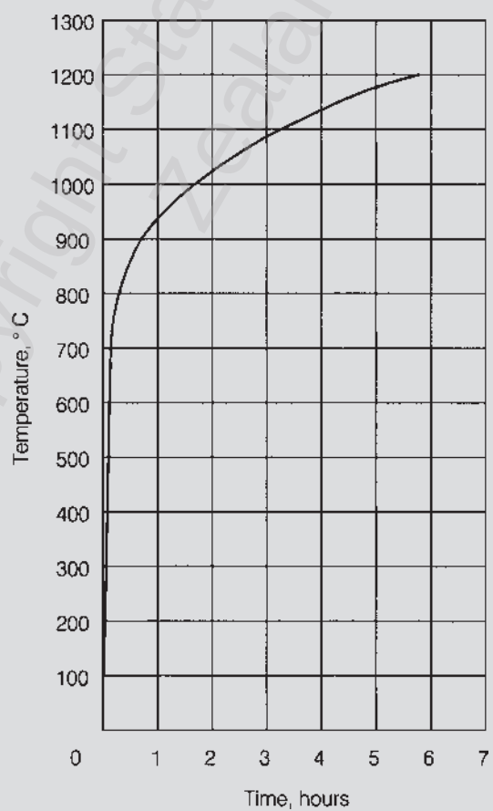
Figure 5.1 – Standard furnace temperature-time curve
