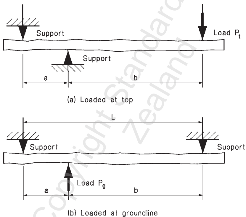
Figure C1 – Schematic plan diagram for proof test loading of round construction piles and poles
