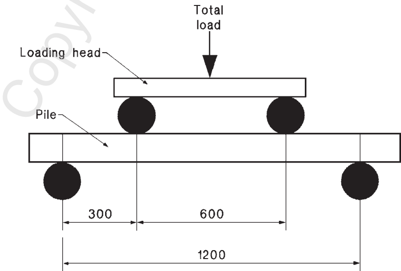
Figure B1 – Schematic plan diagram for testing house piles
