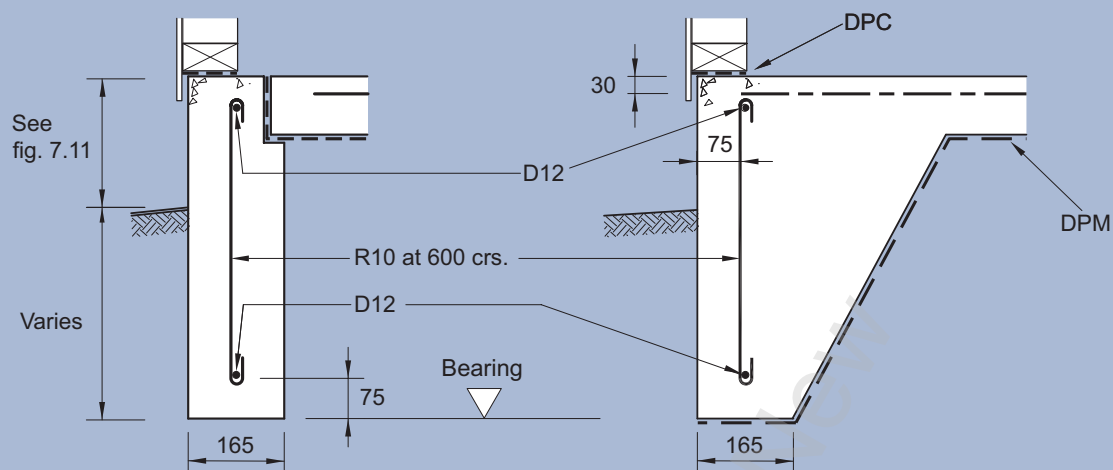
(A) DIMENSIONS & REINFORCING FOR SINGLE STOREY
