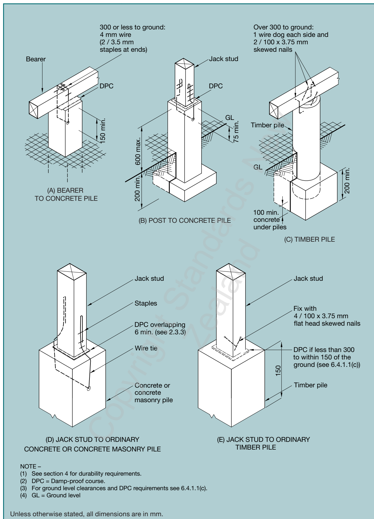
Figure 6.3 – Fixing of bearers and jack studs to ordinary piles (see 6.5.2 and 2.3.3)
