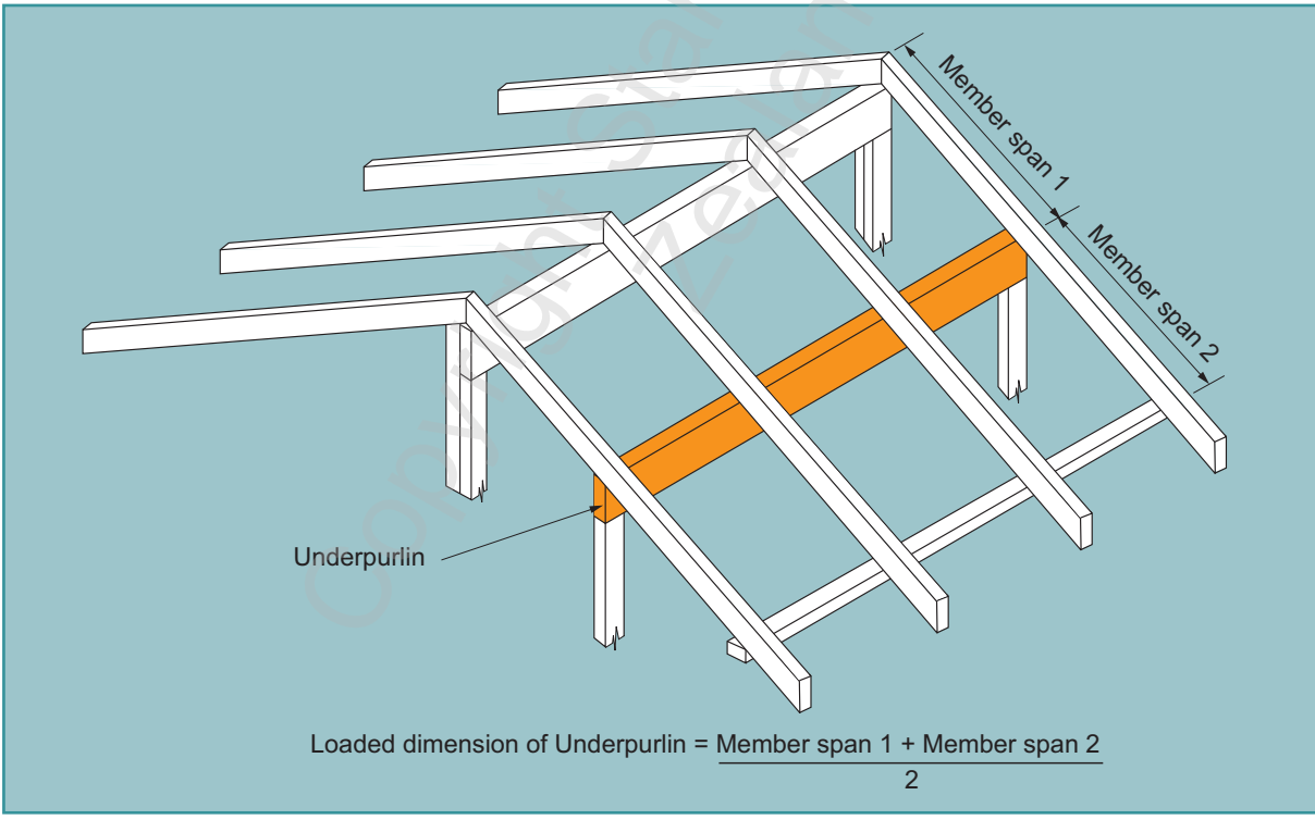
(H) UNDERPURLIN
