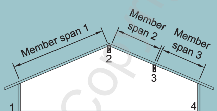
(E) RAFTERS SUPPORTED ON BEAMS OR WALLS
