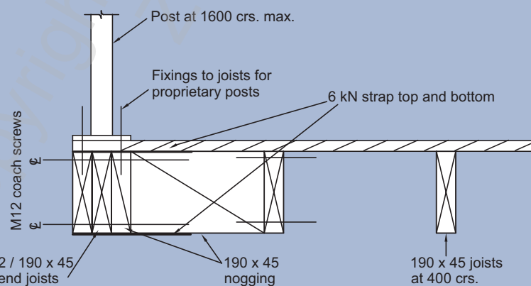
SECTION VIEW AT NOGGING
