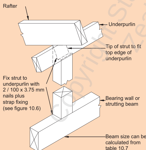
(B) PLUMB STRUT (Perpendicular to ceiling plane)
