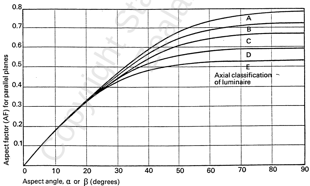
Fig. E7 ASPECT FACTORS FOR PARALLEL PLANES
