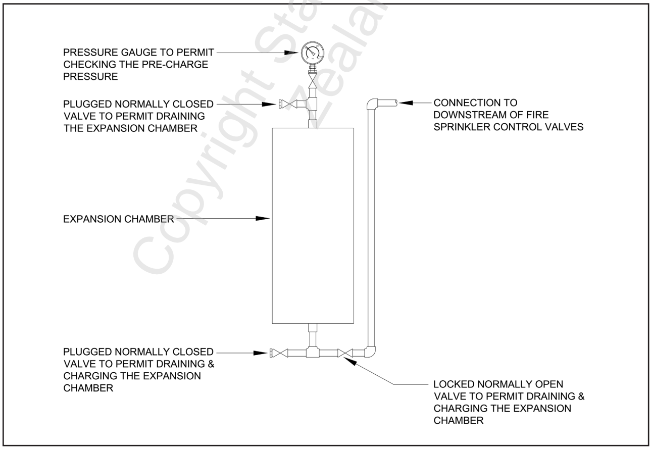
Figure L1 – Gas over water expansion chamber
