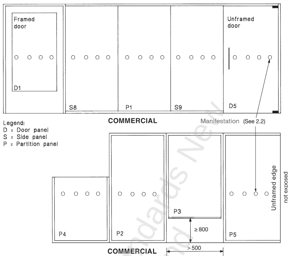
Figure A2 – Examples of internal partitions
