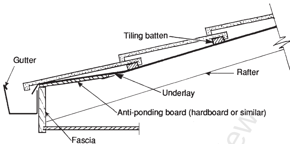
Figure 3 – Anti-ponding board
